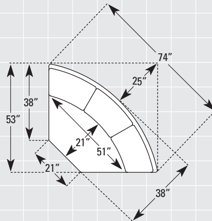
3xx1-53 SEMI-ATTACHED BACK WEDGE OVERALL HEIGHT: 37"
