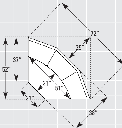
3xx2-53 PULLOVER BACK WEDGE OVERALL HEIGHT: 35"
