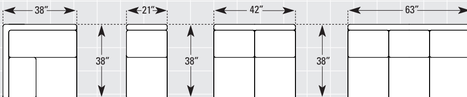
ITEM #32 CORNER CHAIR INSIDE LENGTH: 21"
